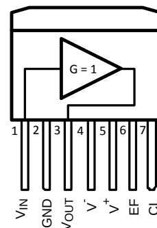
Figure 2. 7-Pin DDPACK(A)
